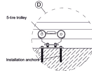
Gate pole foundation of concrete, class min. B15. Foundation depth min. 80cm.
