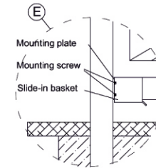
Gate pole foundation of concrete, class min. B15. Foundation depth min. 80cm.
