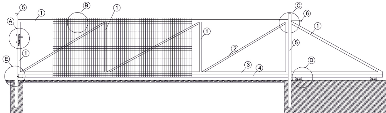
Gate pole foundation of concrete, class min. B15. Foundation depth min. 80cm.
